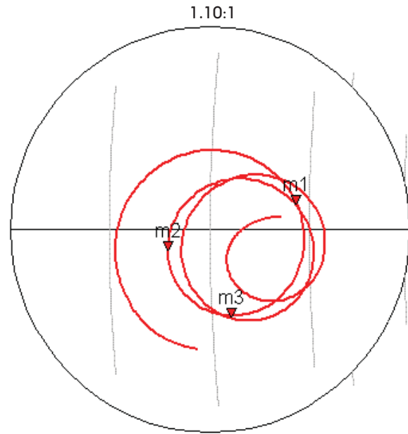
106.3 MHz Typical Smith Chart
