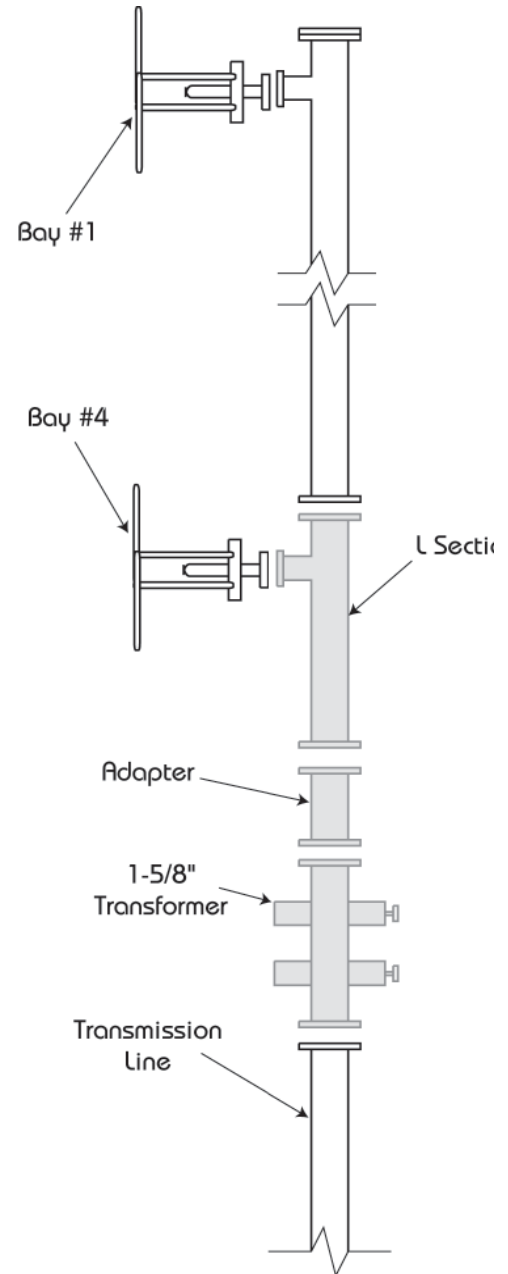
Figure 1. Antenna Assembly Before Conversion (shaded indicates parts removed)
